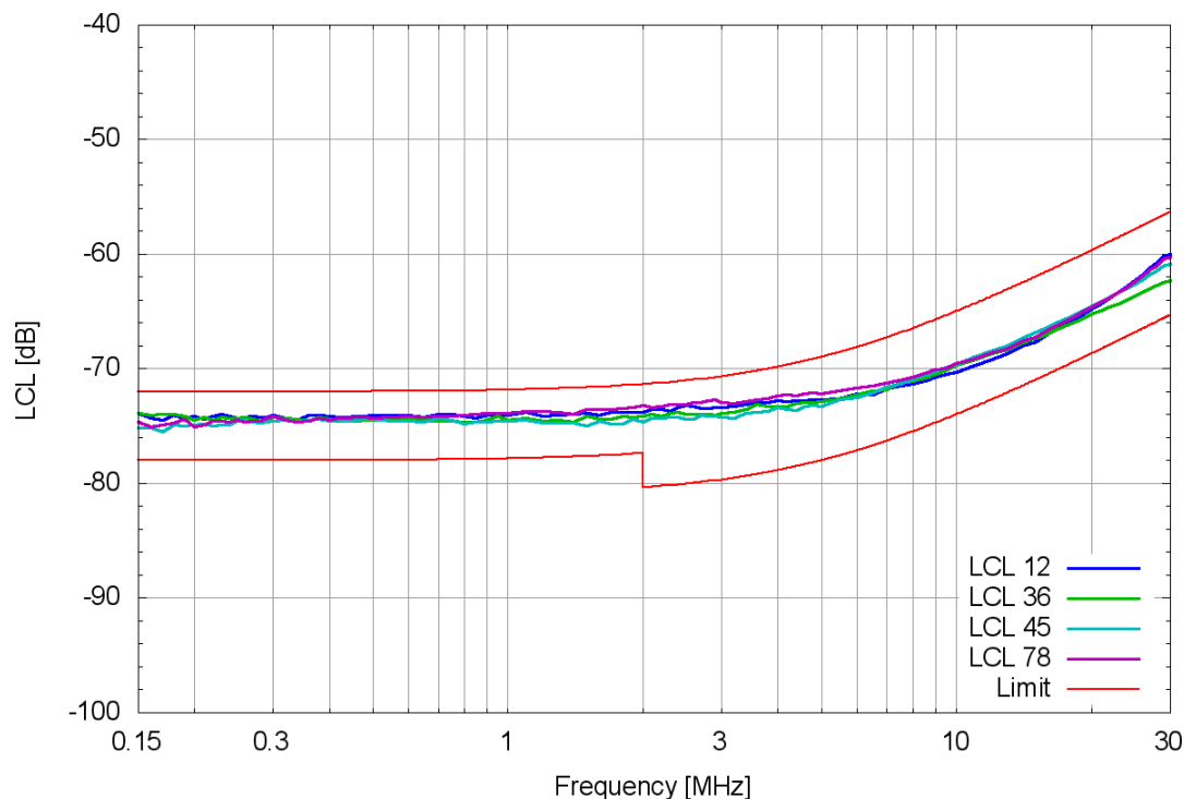
Longitudinal Conversion Loss (LCL)
