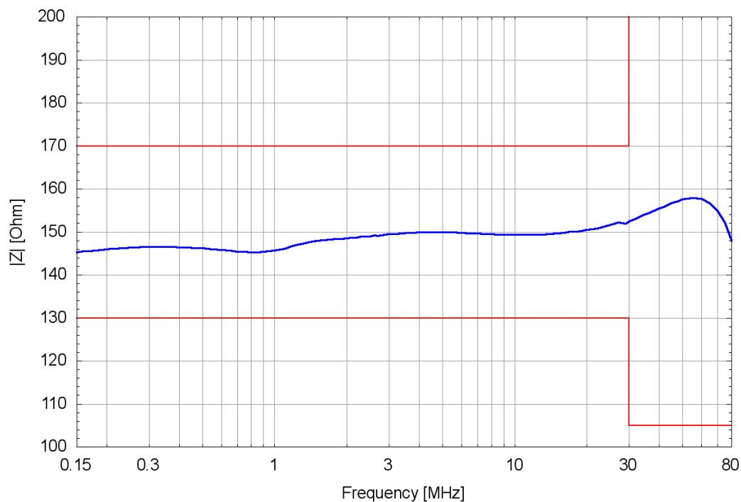
Common Mode Impedance (Magnitude) at EuT-Terminals
