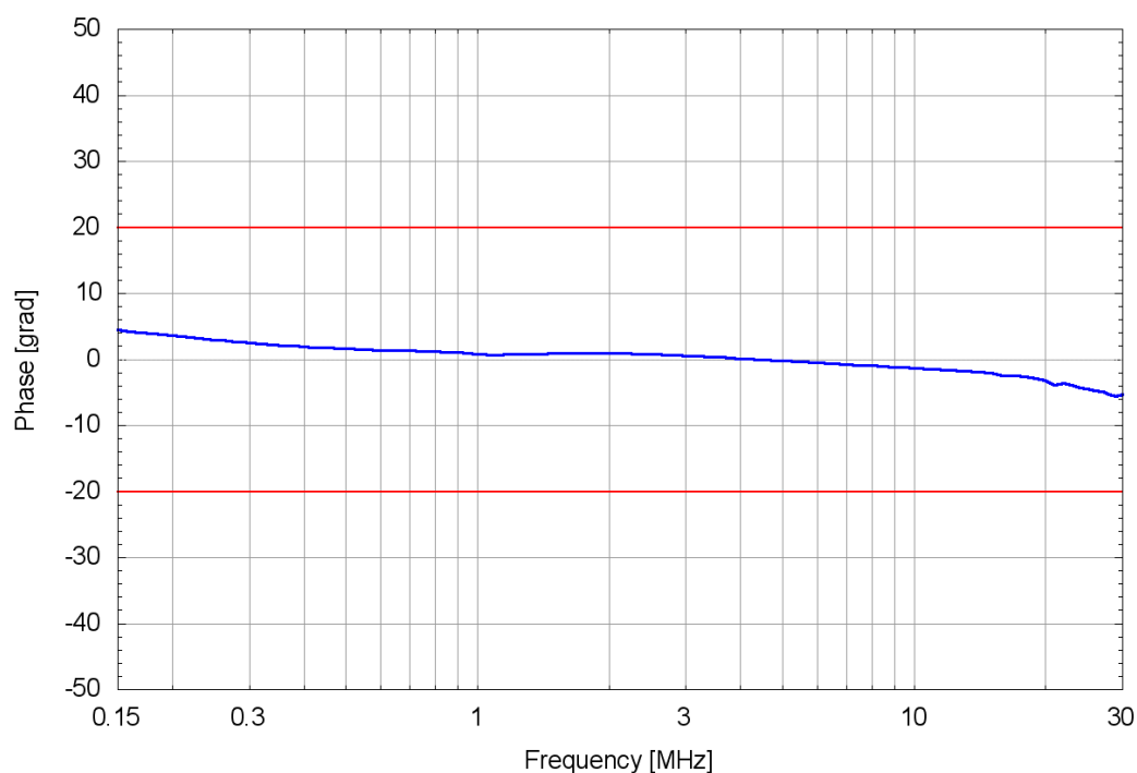
Common Mode Impedance (Phase) at EuT-Terminals
