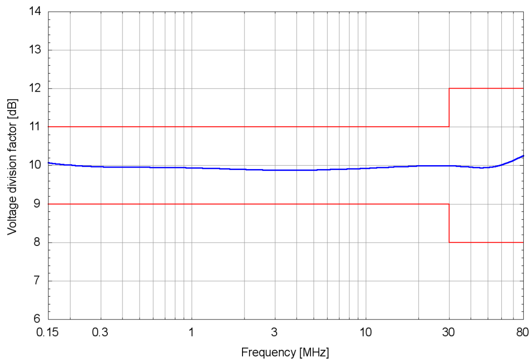
Transmission EuT to Measurement Port
